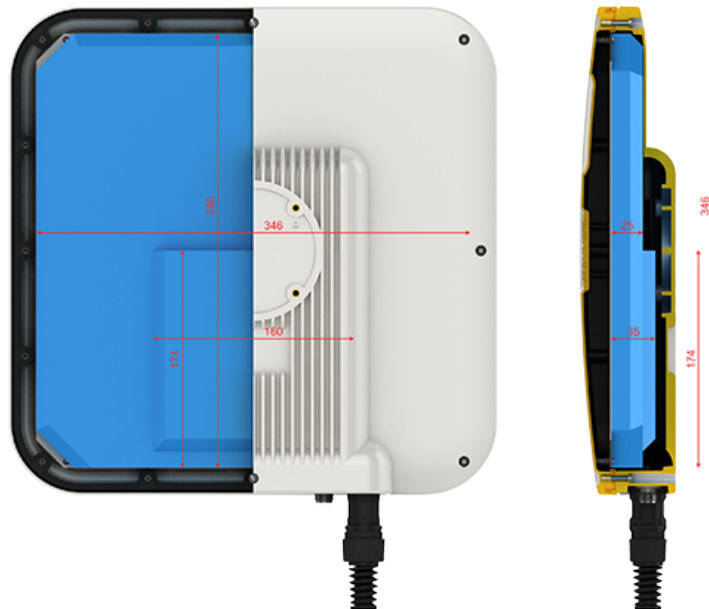
Inner dimensions WiBOX Large Slim
