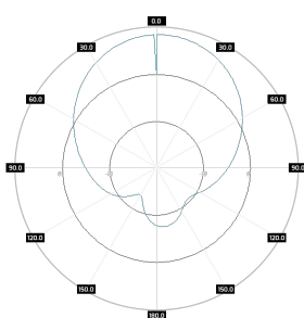
PA M0809-8X Port 1, azimuth
