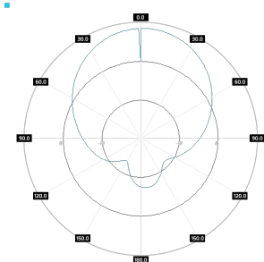
PA M0809-8X Port 2, elev.
