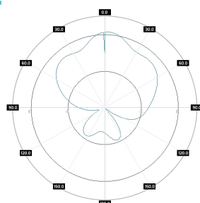
PA MMB0727-8X 2100Mhz, port 2, azimuth
