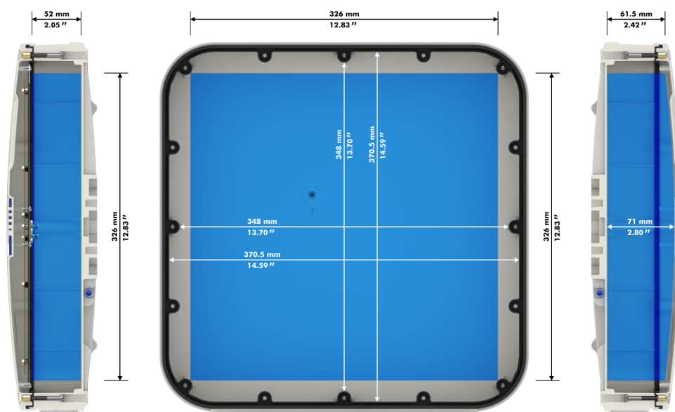
Inner dimensions WiBOX Large
