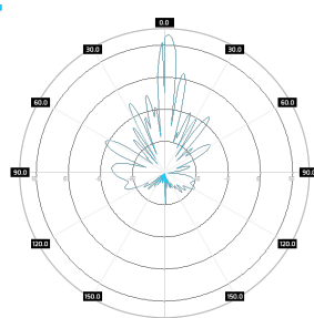
Elevation Port 1, 3800 MHz
