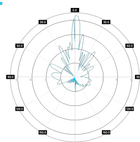
Elevation Port 2, 3800 MHz
