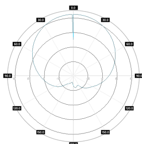
Azimuth Port 2, 3800 MHz
