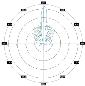
Elevation Port 1, 3500 MHz
