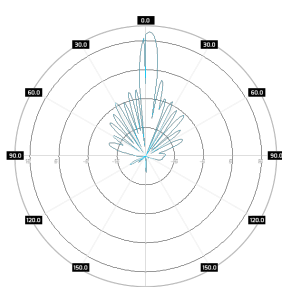
Elevation Port 2, 3500 MHz
