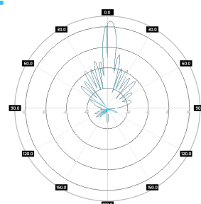
Elevation Port 2, 3300 MHz
