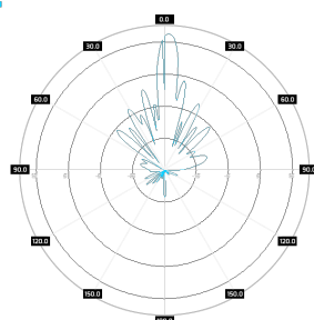
Elevation Port 1, 3300 MHz
