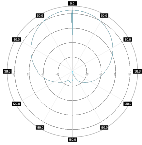
Azimuth Port 1, 3800 MHz
