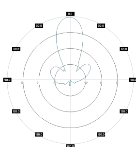
PA M47-20X Port 1, azimuth
