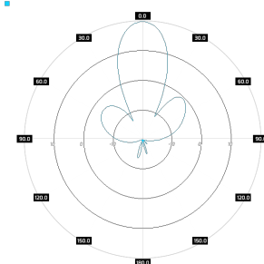
PA M47-20X Port 1, elev
