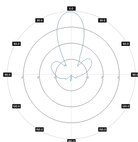
PA M47-20X Port 1, azimuth
