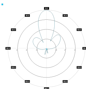
PA M47-20X Port 1, elev
