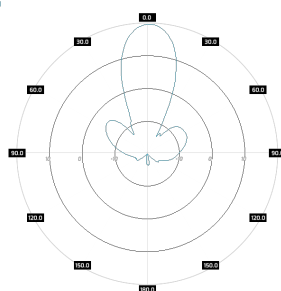
PA M47-20X Port 2, azimuth
