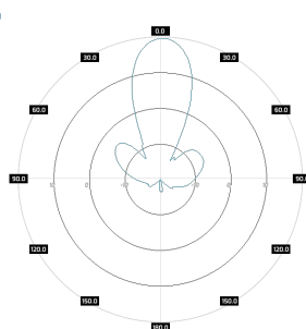
PA M47-20X Port 2, azimuth
