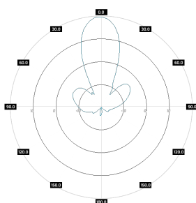
PA M47-20X Port 1, azimuth
